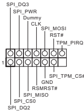
SPI_TPM_J1
